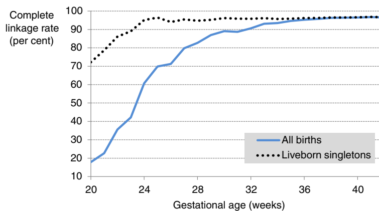
Figure 2 Linkage rate for complete group by gestational age (weeks). Complete linkage rate (number of birth records linked to both a mother and infant hospital admission birth record as a percentage of all birth records) by gestational age for all births (blue line) and liveborn singletons (dotted black line).
