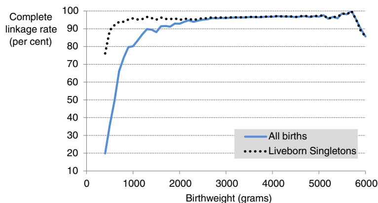
Figure 3 Linkage rate for complete group by birth weight (grams). Complete linkage rate (number of birth records linked to both a mother and infant hospital admission birth record as a percentage of all birth records) by birthweight for all births (blue line) and liveborn singletons (dotted black line).
